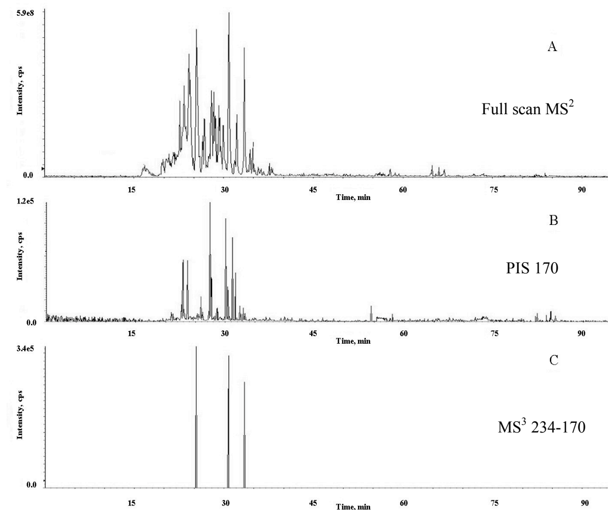
Fig.2.7 In the panel A it is showed the total ion current of a full scan LC-MS 2 of a nitrated BSA/BSA trypsin digest. Panel B: PIS of nitrated BSA/BSA peptide mixture after dansyl labelling. About 73% of un-desired peptides are not analyzed. The MS 3 chromatogram in panel C shows that by the double selection criteria 100% of un-desired peptides are removed by the spectrometer.
